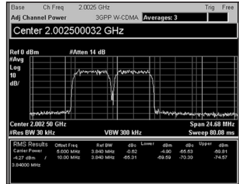
Typical 3GPP 2 carrier test model 1 (64 channels)
